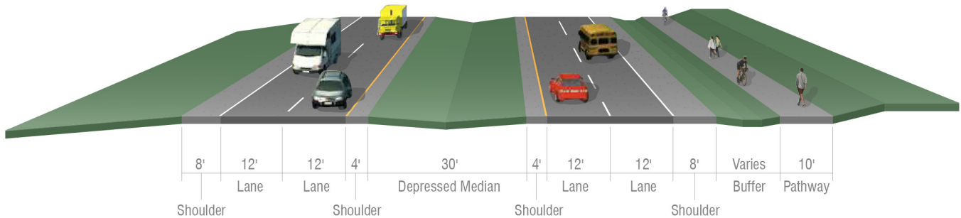
Figure 1: Proposed Typical Section - Looking South
